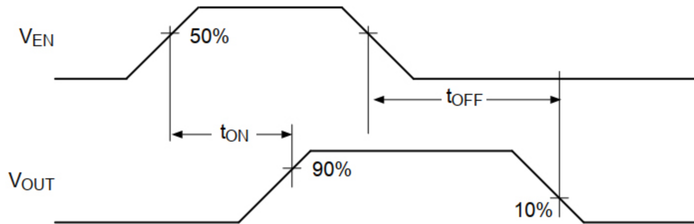
Active-High Switch Delay Time ( XL20x6-1)
