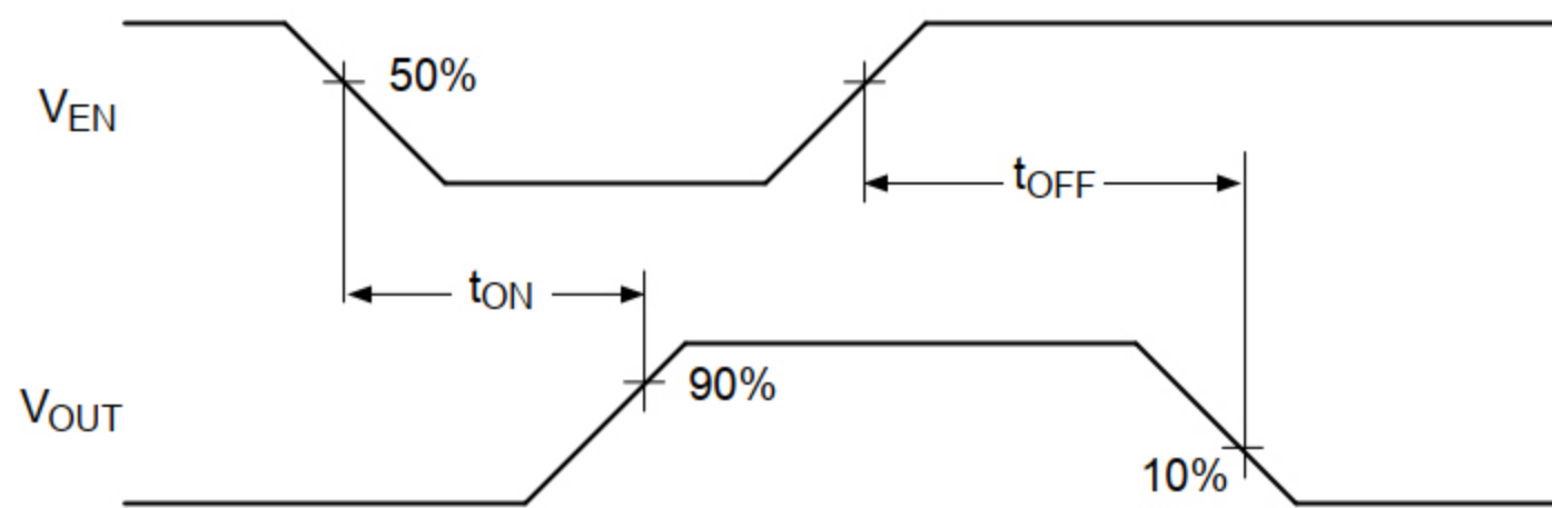
Active-Low Switch Delay Times ( XL20x6-2)
