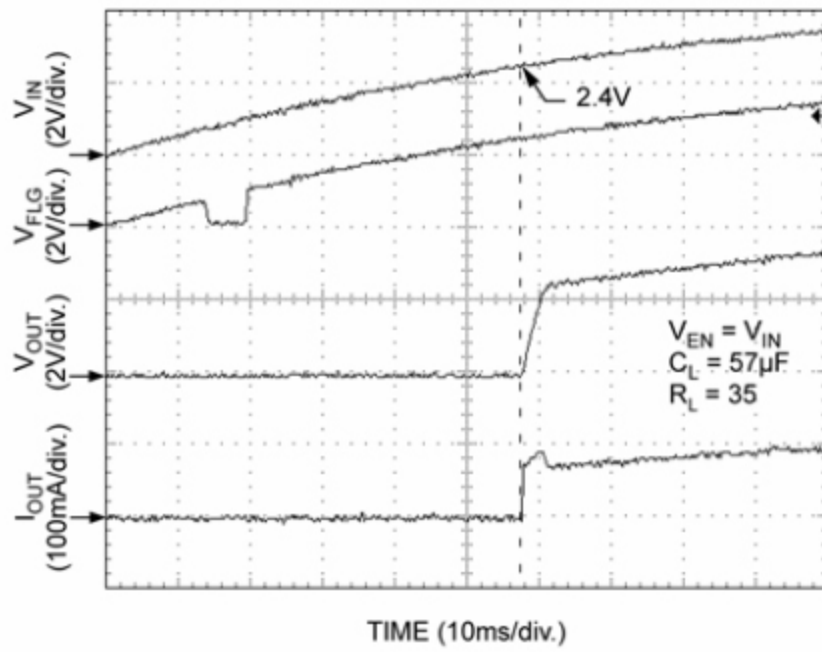
Turn-On/Turn-Off ( XL2026-1)
