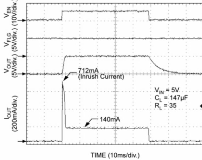
Turn-On/Turn-Off ( XL2026-1)
