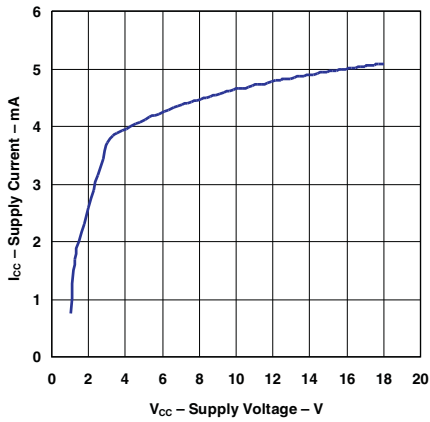
Supply Current vs Supply Voltage (T A = 25°C)
