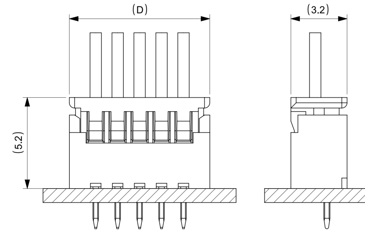
① 嵌合図 MATED CONNECTORES
