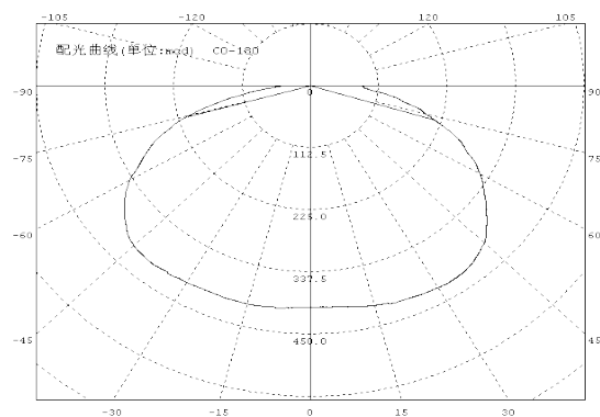
Directive Characteristics
