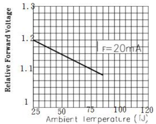
Fig. 6 Forward Voltage vs. Ambient Temperature (Tj)
