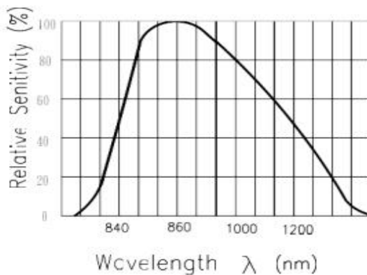
Fig.5 Spectral Sensitivity
