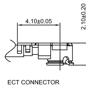
ECT CONNECTOR
