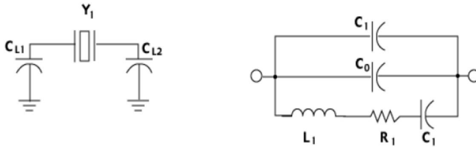
Figure 4. Crystal load capacitors and equivalent parallel load.
