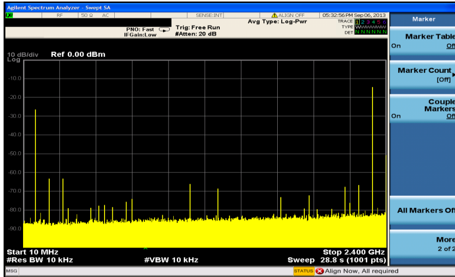
图 14 单音信号频谱, f_{OUT}=2.31GHz , f_{DAC}=2.4GSPS
