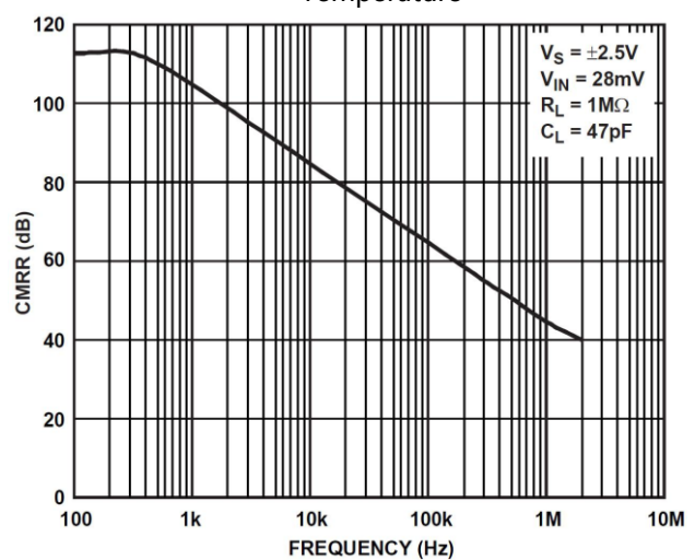
14. CMRR vs. Frequency
