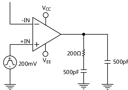
Figure 55. Snubber Network
