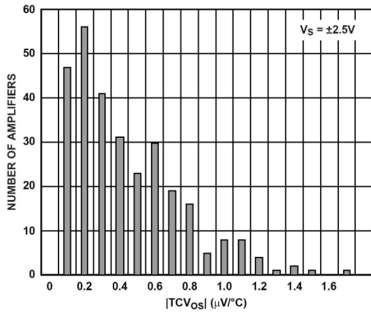
Figure 5. |TCVos| Distribution
