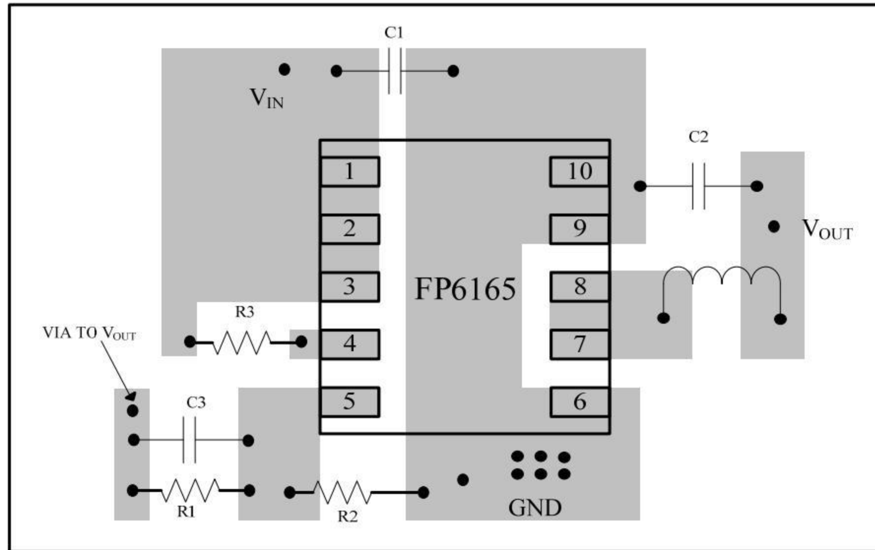
Suggested Layout for DFN-10L / MSOP-10L
