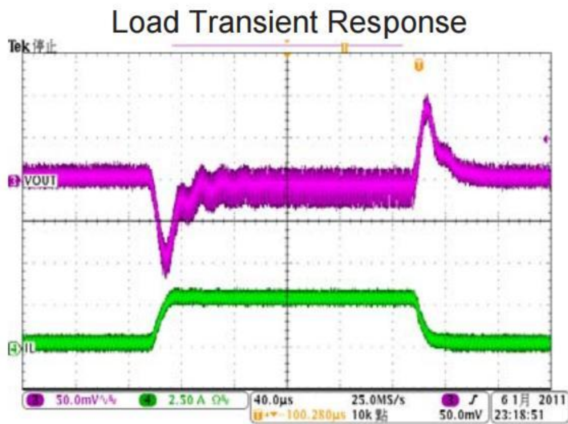
I_{LOAD}: 300mA \sim 3A
