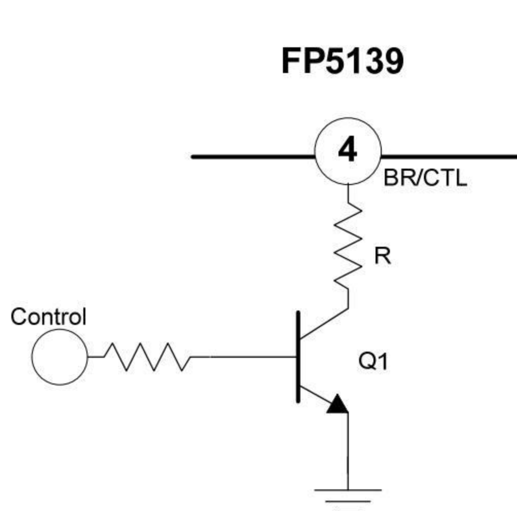
Figure 13 Output Transistor Driving Control Circuit
