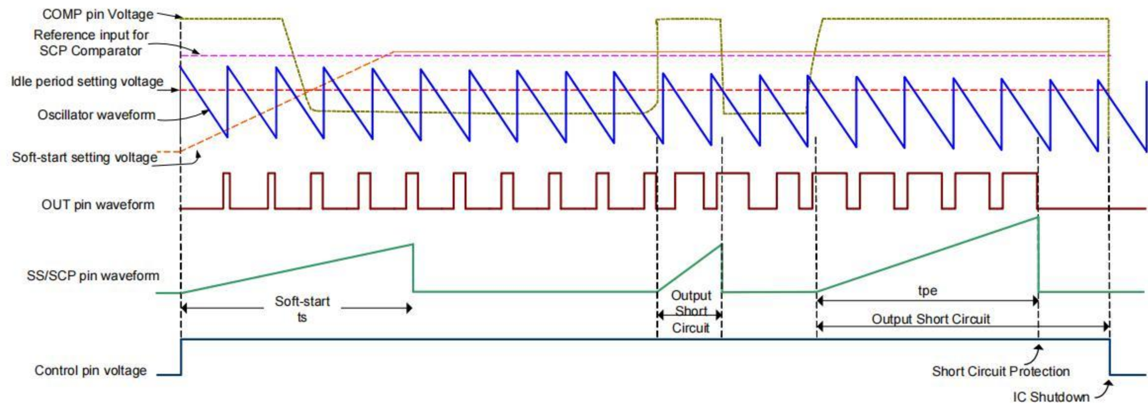
Figure18 FP5139 Timing Diagram
