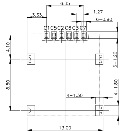
RECOMMENDED PCB LAYOUT TOP VIEW (TOLERANCE:±0.05) RECOMMENDED MATAI MASK T=0.12MM
