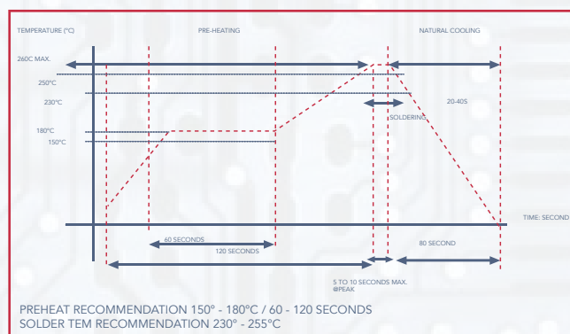
WAVE SOLDERING (FLOW SOLDERING)
