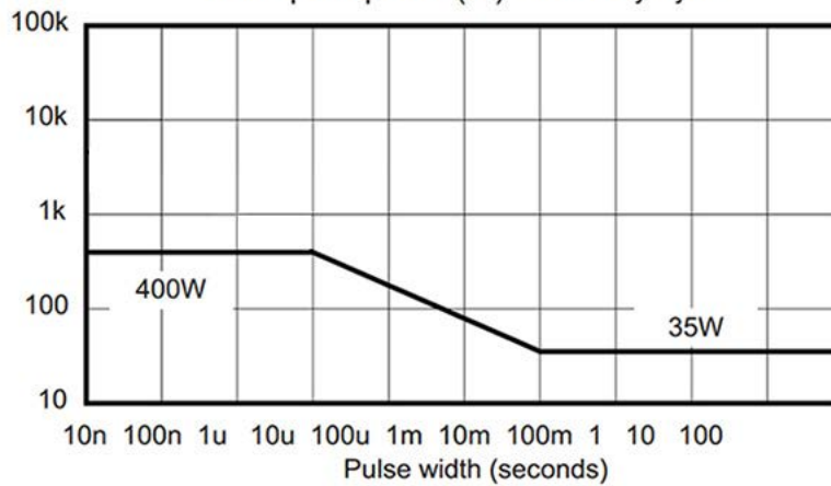
Pulse peak power (W) - 0.01 Duty Cycle
