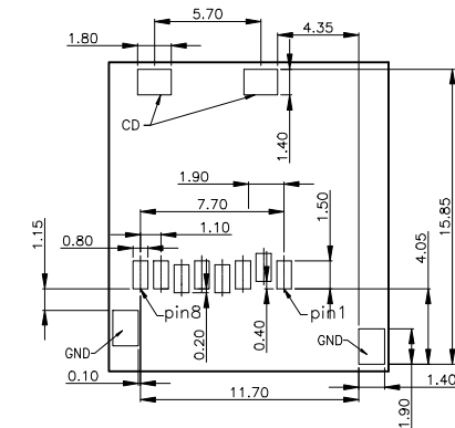
RECOMMENDED P.C.B HOLE LAYOUT COMPONENT SIDE VIEW(TOLERANCE: +/-0.05)
