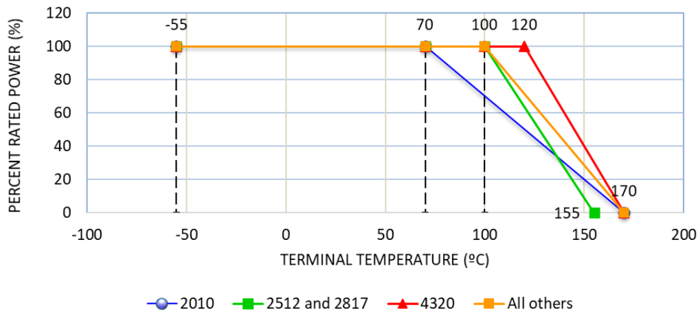
Power Derating Curve:
