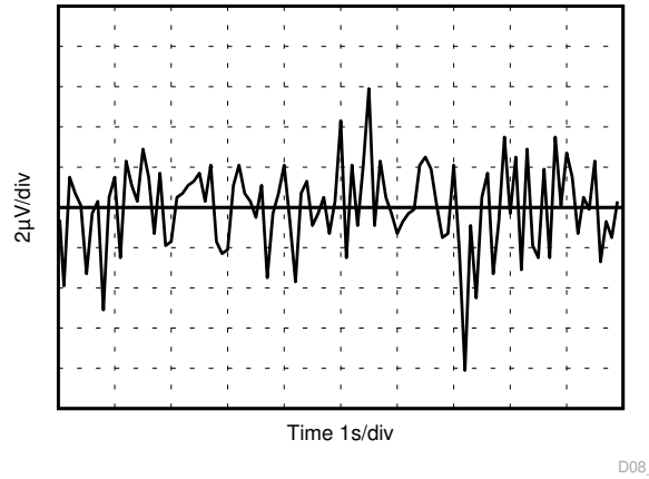
图 8-5. 0.1-Hz to 10-Hz Noise ( V_{OUT} )
