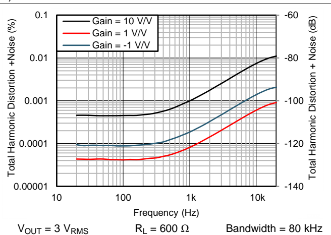
图 8. THD+N Ratio vs Frequency
