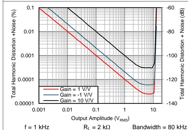
图 9. THD+N Ratio vs Output Amplitude
