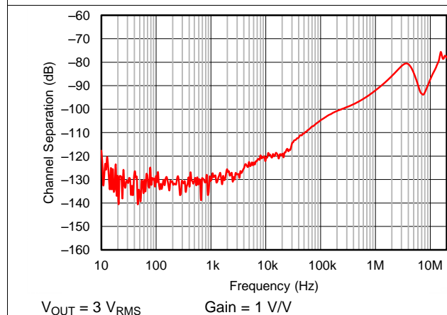
图 11. Channel Separation vs Frequency
