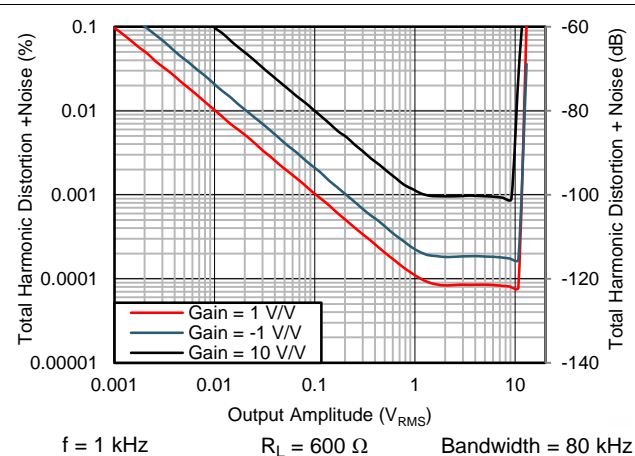
图 10. THD+N Ratio vs Output Amplitude
