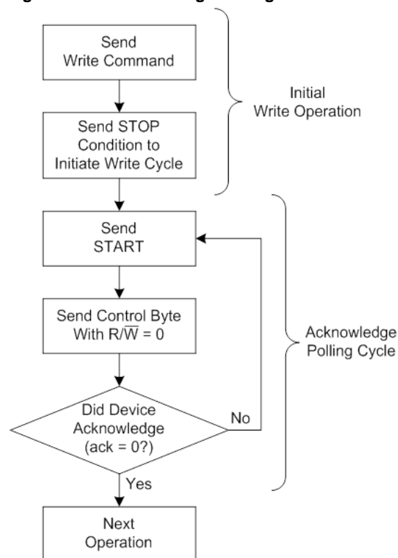
Figure 9-1. Acknowledge Polling Flow
