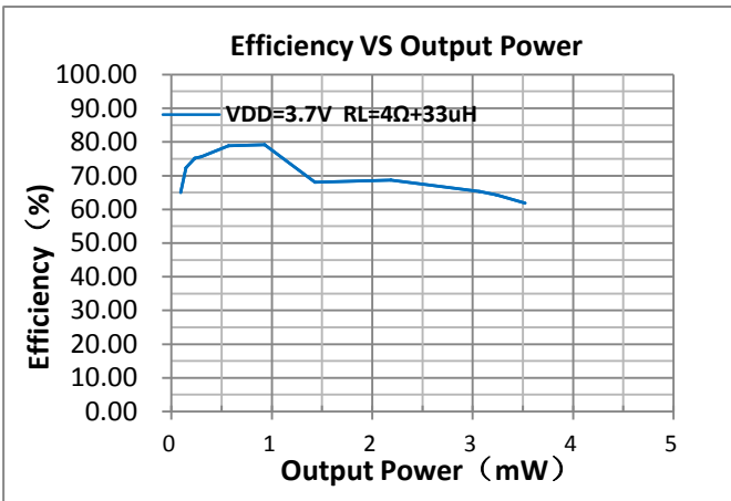
图3: Efficiency VS Output Power
