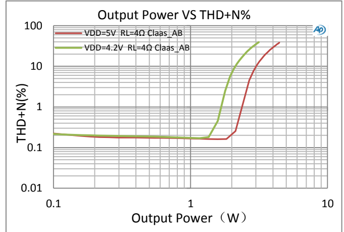
图2: Output Power VS THD+N
