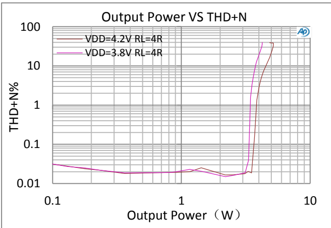
图1: Output Power VS THD+N
