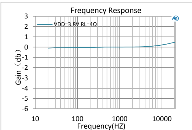
图5: Frequency Response
