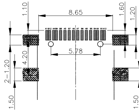
PCB LAYOUT(Recommend) (General Tolerance:±0.05)
