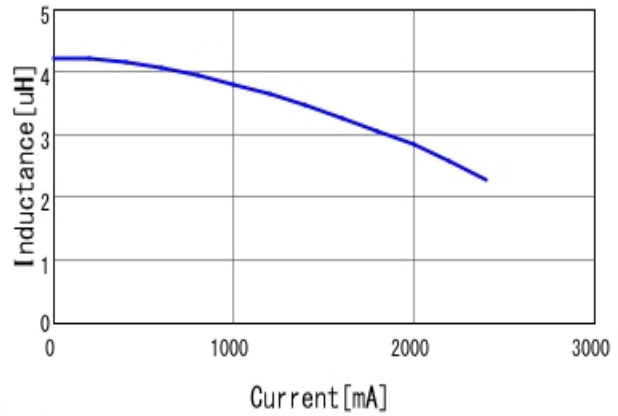
■ 1239AS-H-4R7M L-Current 20degC
