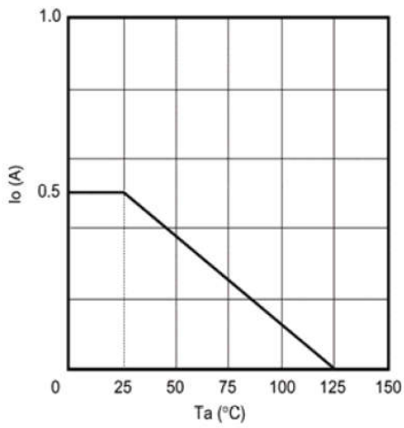
Fig.4 Derating curve
