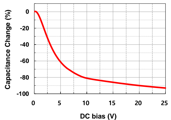
- Capacitance Change(%) with DC bias
