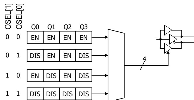
Figure 2. Output Enable Map Operation
