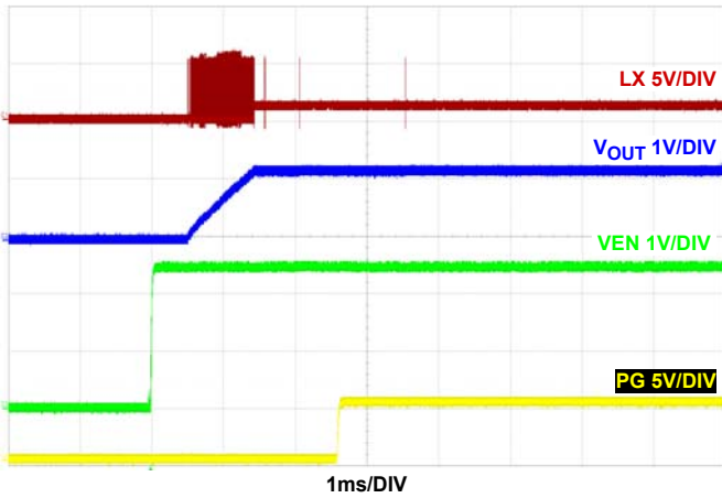
FIGURE 21. START-UP AT NO LOAD F_{SW} = 2\text{MHz} , V_{IN} = 5\text{V} , MODE = PFM, T_A = +25^\circ\text{C}
