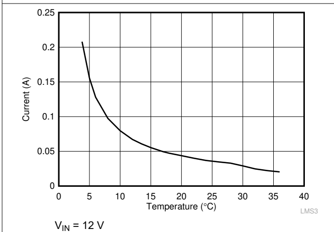
Figure 7-5. Short Circuit Average Input Current for LMS3635-Q1
