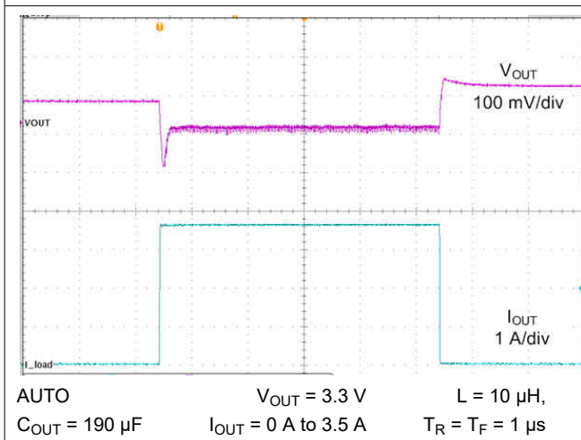
Figure 9-27. Load Transient
