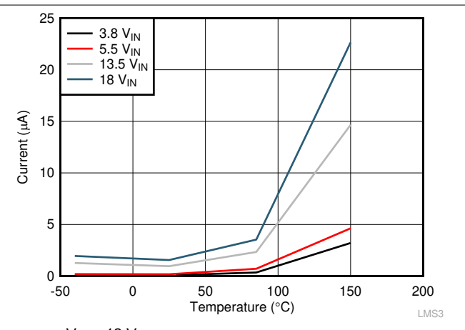
Figure 7-6. Shutdown Current
