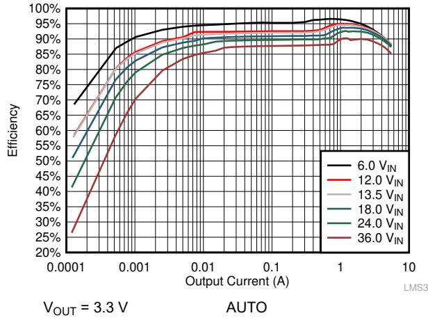
Figure 9-17. Efficiency
