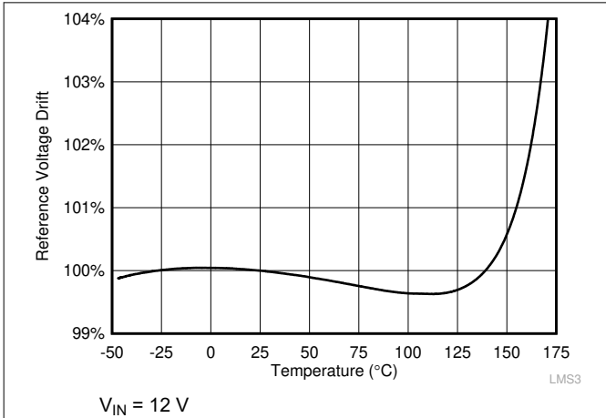
Figure 7-1. Reference Voltage Drift
