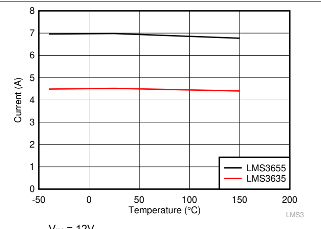
Figure 7-4. Low-Side/Valley Current Limit for LMS36x5-Q1
