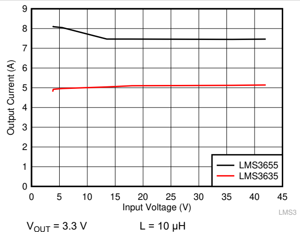
Figure 9-26. Output Current Level for Overcurrent Protection Trip
