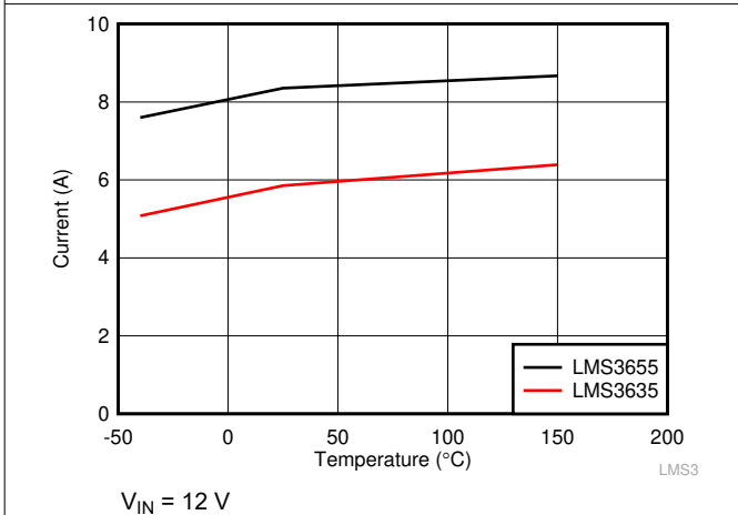
Figure 7-3. High-Side/Peak Current Limit for LMS36x5-Q1
