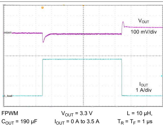
Figure 9-28. Load Transient
