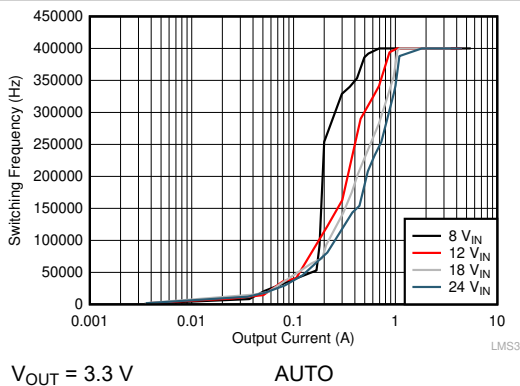
Figure 9-25. Switching Frequency vs Load Current
