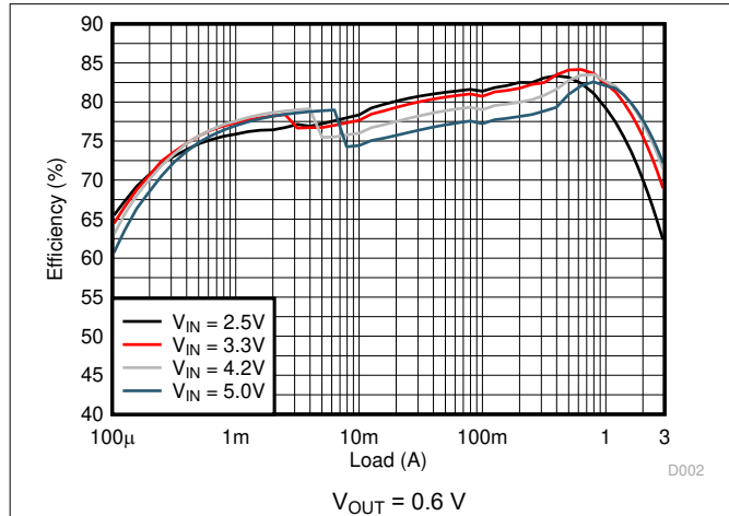
Figure 9-3. Efficiency
