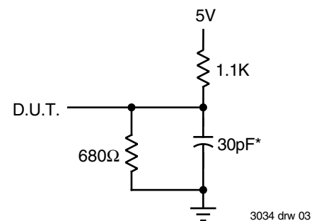
Figure 1. Output Load
