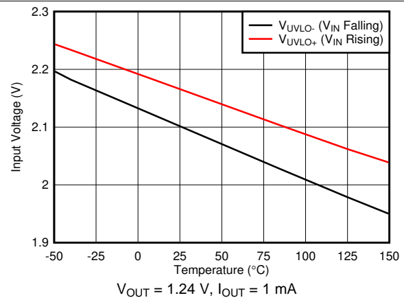
Figure 14. UVLO Thresholds vs Temperature
