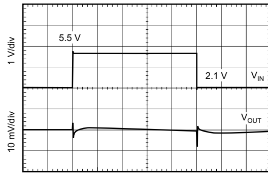
V_{OUT} = 1.8\text{ V} , I_{OUT} = 300\text{ mA} , slew rate = 1\text{ V}/\mu\text{s}
