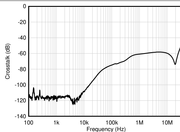
Figure 7-46. Channel Separation
