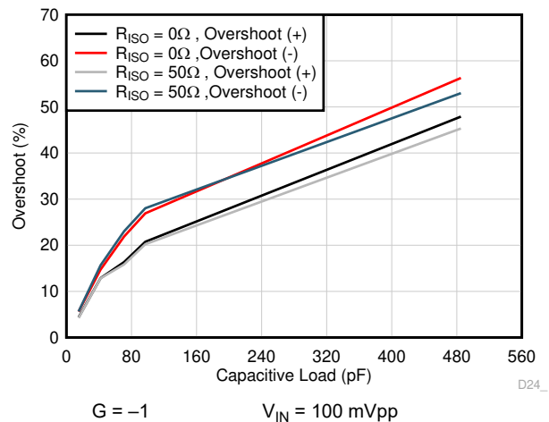
Figure 7-30. Small Signal Overshoot vs Capacitive Load
