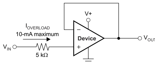
Figure 8-6. Input Current Protection
