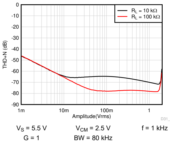
Figure 7-25. THD + N vs Amplitude
