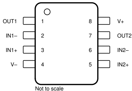
Figure 6-6. TLV9042 D, DDF, DGK, and PW Package 8-Pin SOIC, SOT-23 8, VSSOP, and TSSOP Top View
