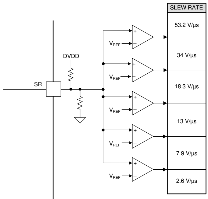
Figure 7-8. SR Block Diagram
