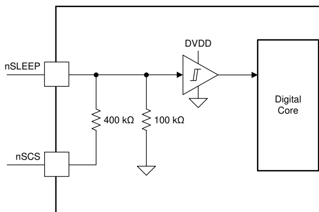
Figure 7-11. nSCS and nSLEEP Circuit
