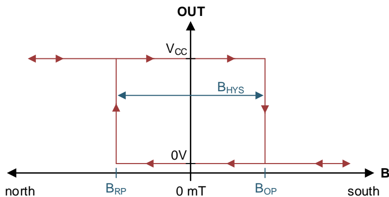
Figure 9. Device Functionality
