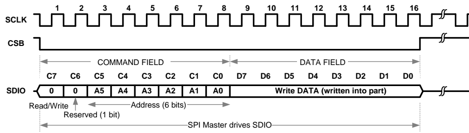
Figure 37. Serial Interface Protocol (Write Operation)
