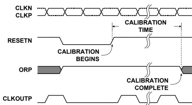
FIGURE 22. CALIBRATION TIMING
