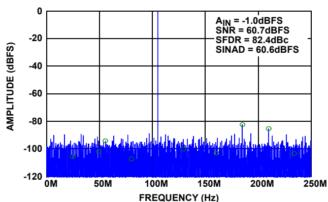
FIGURE 15. SINGLE-TONE SPECTRUM AT 105MHz
