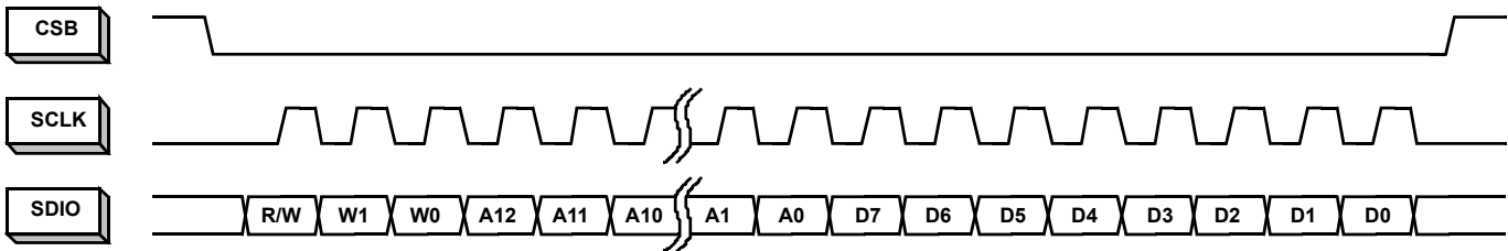
FIGURE 33. MSB-FIRST ADDRESSING
