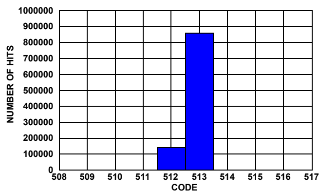
FIGURE 14. NOISE HISTOGRAM
