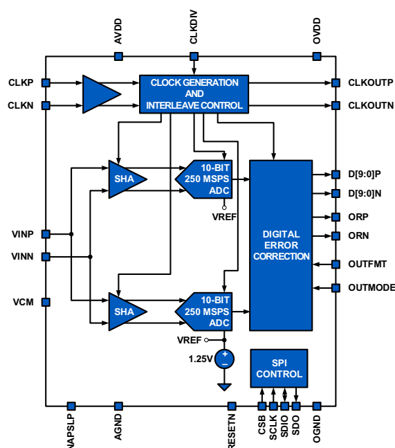
FIGURE 1. BLOCK DIAGRAM
