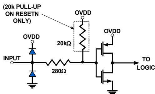
FIGURE 44. DIGITAL INPUTS
