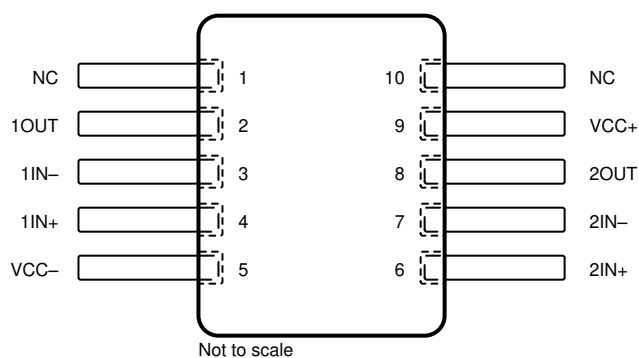
Figure 5-5. TL072x U Package 10-Pin CFP Top View
