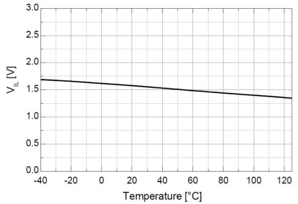
Figure 12. Logic Low Input Voltage vs. Temperature
