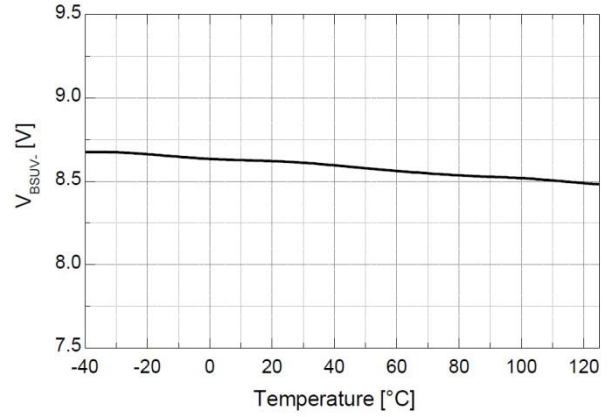
Figure 11. V_{BS} UVLO- vs. Temperature
