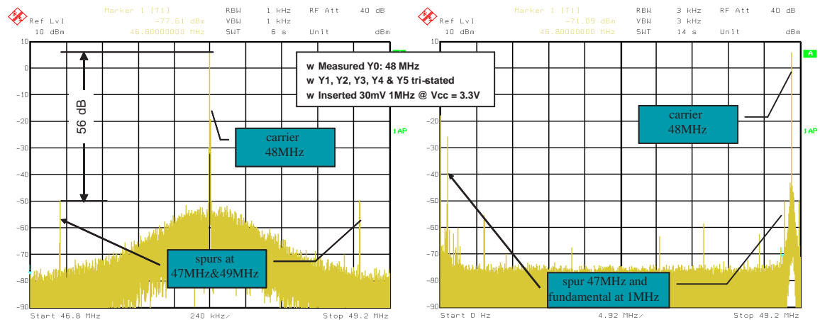
Figure 32. Power Supply Noise Rejection
