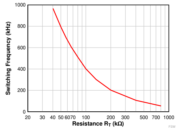
Figure 6-22. Channel Switching Frequency F_{SW} vs R_T Resistance
