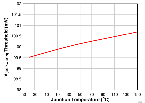
Figure 6-20. V_{(CSP - VCSN)} Voltage vs Junction Temperature
