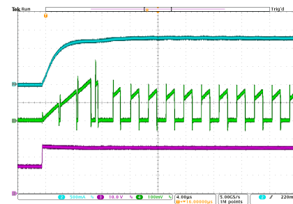
CH2: Buck-Boost I_{LED} CH4: Buck-Boost switch current sense voltage CH3: Buck-Boost LED+ voltage (3xLED)
