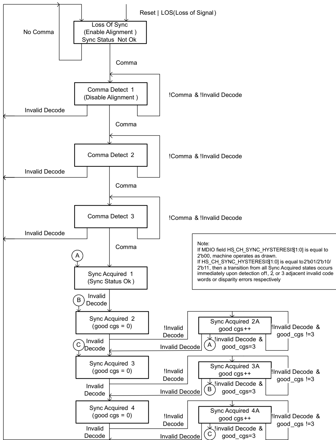
Figure 5-3. Channel Synchronization Flowchart
