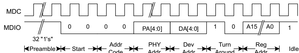
Figure 5-38. CL45 - Management Interface Extended Space Address Timing
