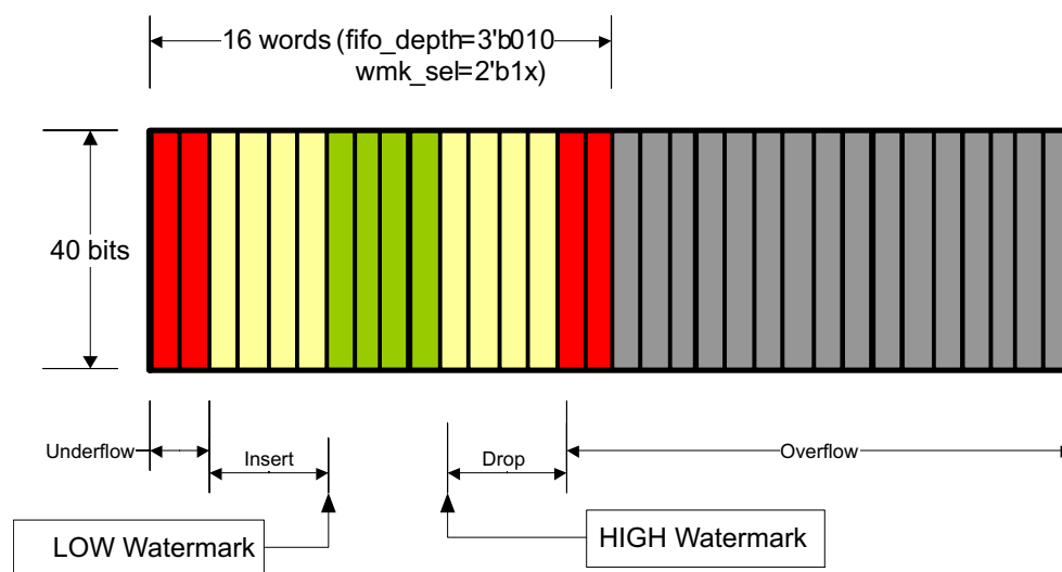
Figure 5-28. Organization of the XAUI CTC FIFO (16-Deep, High Watermark)
