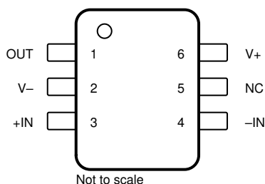
Figure 5-3. OPA991S DBV and DRL Package (A) 6-Pin SOT-23 and SOT-563 Top View
