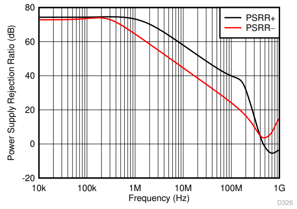
Small-Signal Response
