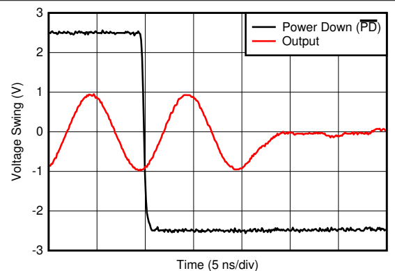
Figure 6-24. Turnoff Transient Response
