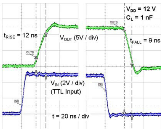
Figure 40. Rise / Fall Waveforms with 1 nF Load
