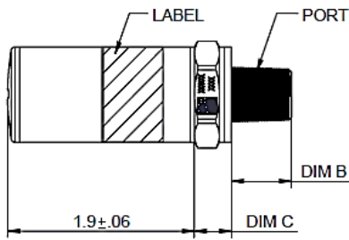
* FOR PRESSURE PORT CODE:5,6,E,F,P,N,W
