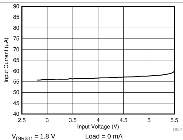
Figure 7. PFM Mode Current Consumption vs Input Voltage, One Regulator Enabled (1+1+1+1-Phase Output)
