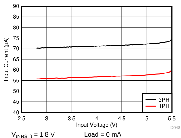
Figure 5. PFM Mode Current Consumption vs Input Voltage, One Regulator Enabled (3+1-Phase Output)
