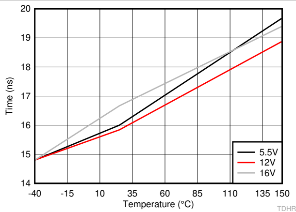
Figure 6-23. HO Rising Propagation Delay (TDHR)
