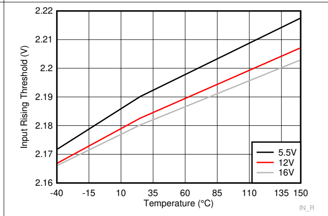
Figure 6-6. Input Rising Threshold
