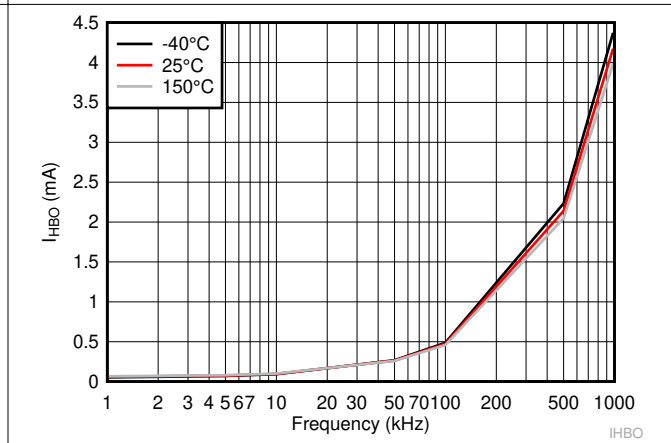
Figure 6-4. HB Operating Current
