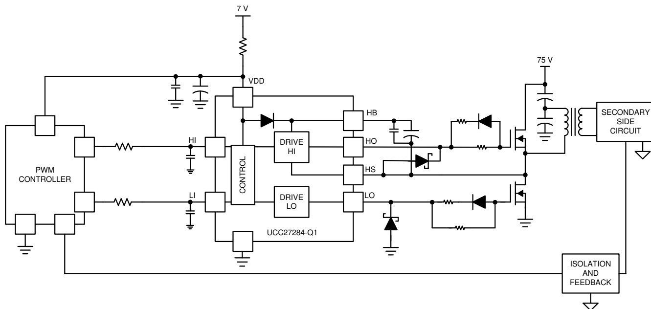
Figure 8-1. Typical Application
