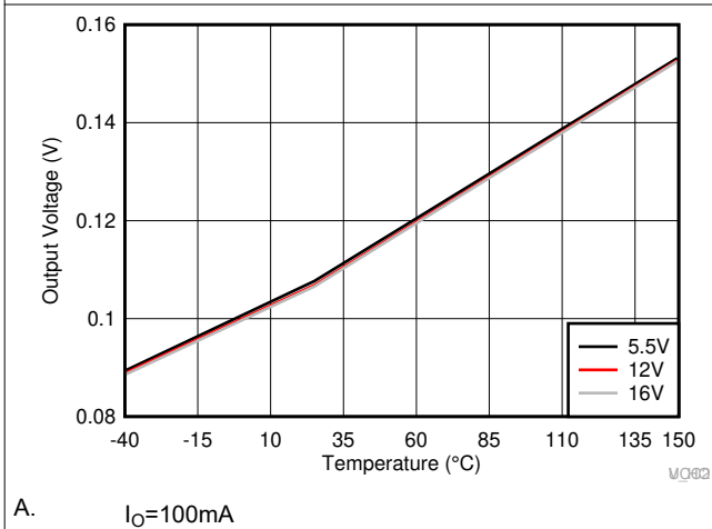
Figure 6-13. LO Low Output Voltage ( V_{LOL} )
