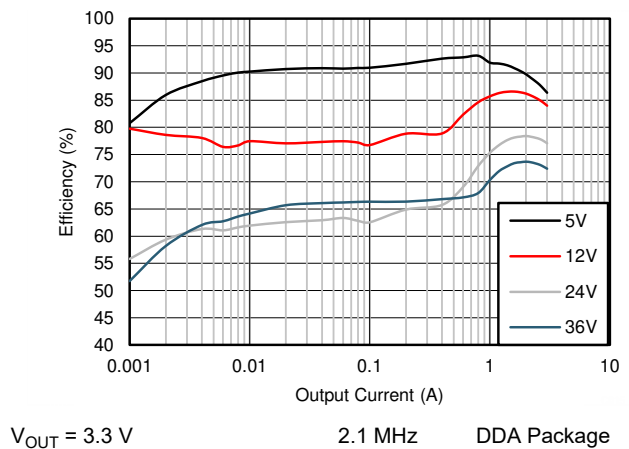
Figure 9-12. Efficiency
