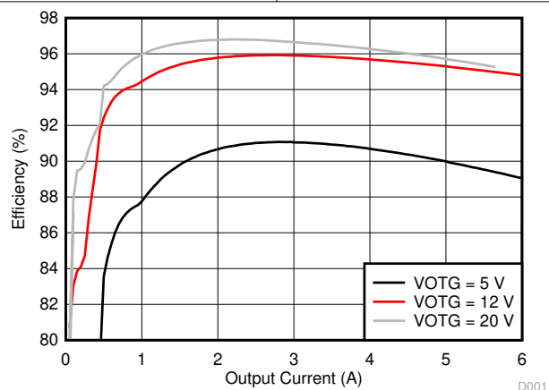
Figure 8-11. OTG Efficiency with 4S Battery
