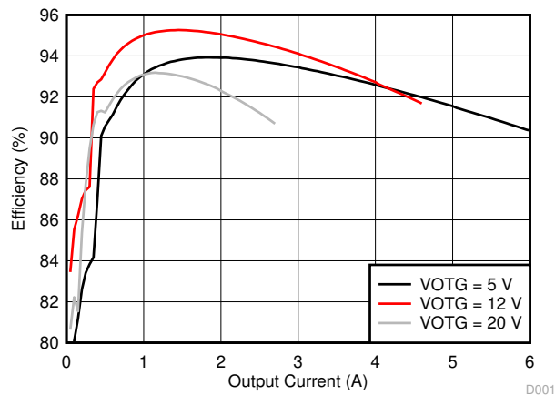
Figure 8-9. OTG Efficiency with 2S Battery
