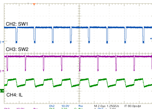
Figure 10-10. Switching During Buck Boost Mode
