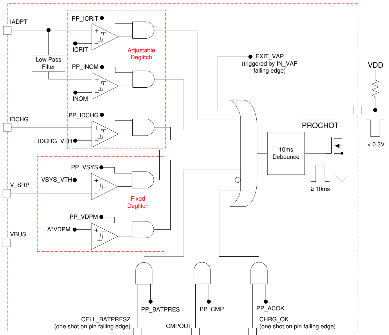
Figure 9-2. PROCHOT Profile
