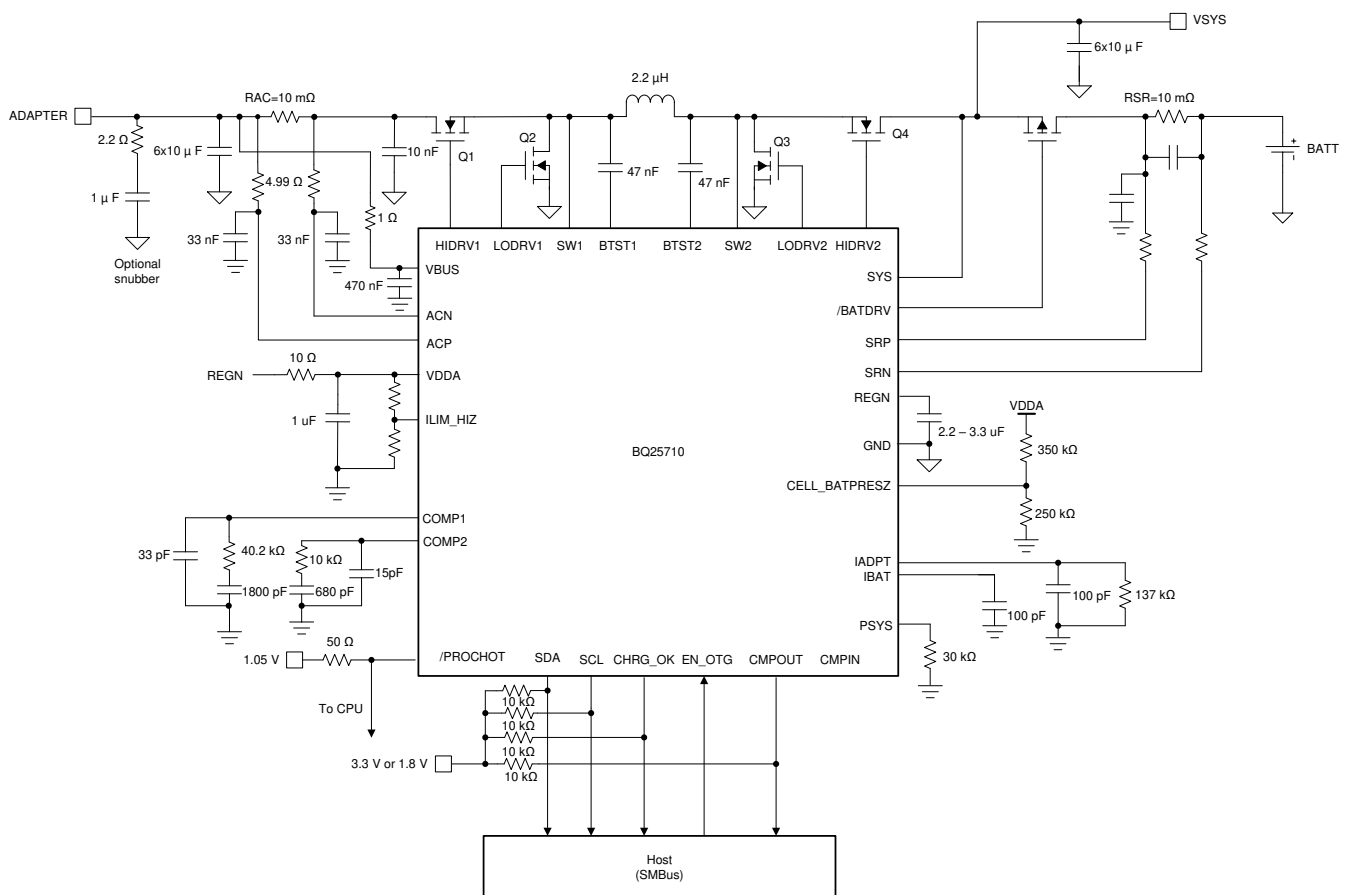
Figure 10-1. Application Diagram
