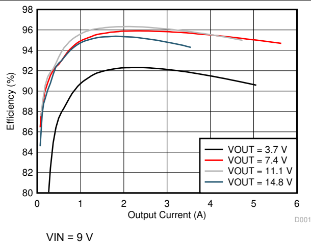
Figure 8-5. System Efficiency
