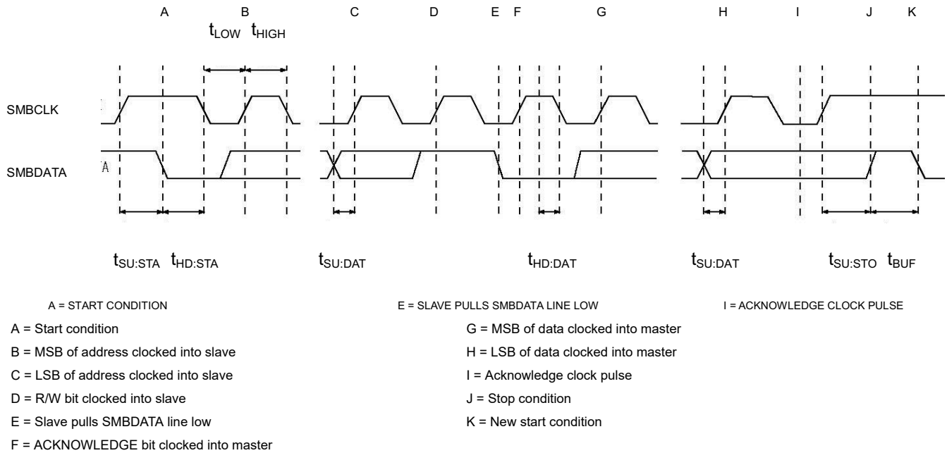
Figure 9-5. SMBus Read Timing
