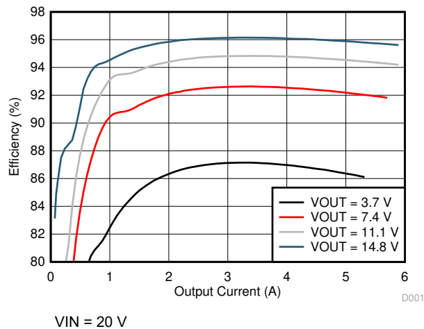
Figure 8-7. System Efficiency
