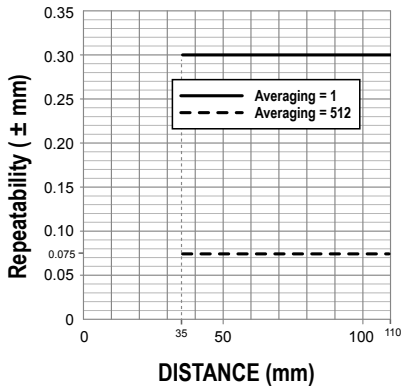
Figure 27. 110 mm Models
