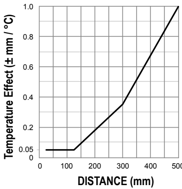
Figure 22. 500 mm Models
