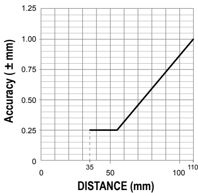
Figure 24. 110 mm Models
