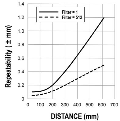
Figure 29. 610 mm Models
